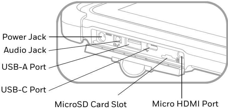
I/O Panel (I/O cover open)
