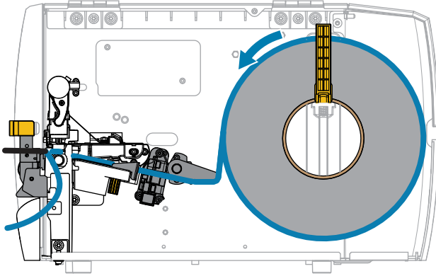
Figure 5 Liner Take-Up Option
